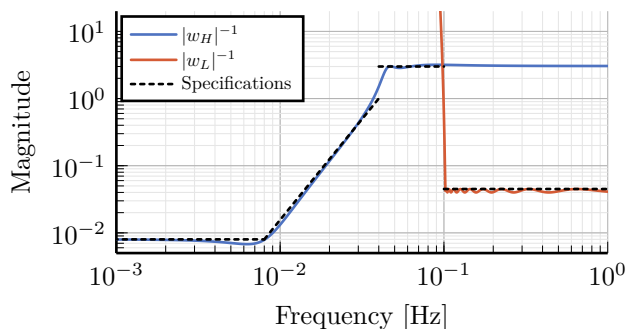
Fig. 9. Specifications and weighting functions magnitudes
