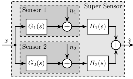
Fig. 1. Sensor fusion architecture
