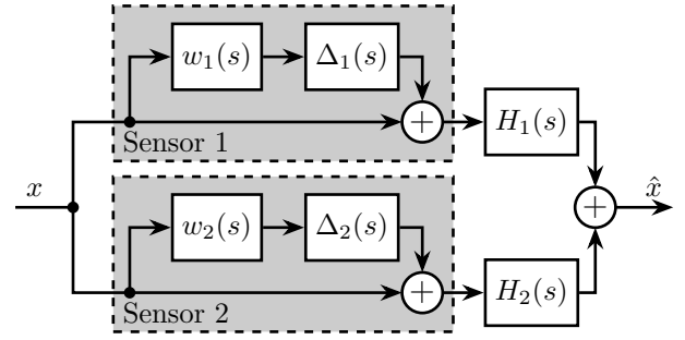
Fig. 2. Sensor fusion architecture with sensor dynamics uncertainty
