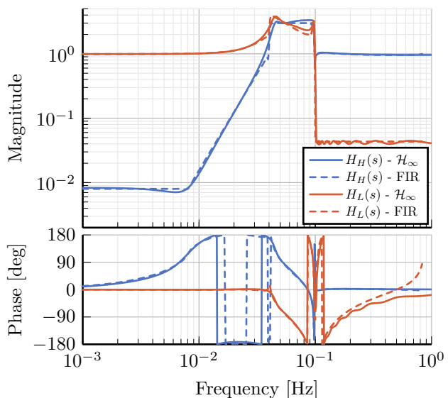
Fig. 10. Comparison of the FIR filters (solid) designed in [10] with the filters obtained with \mathcal{H}_\infty synthesis (dashed)
